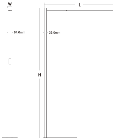
L x W x H: 1056 x 64 x 1950 mm
